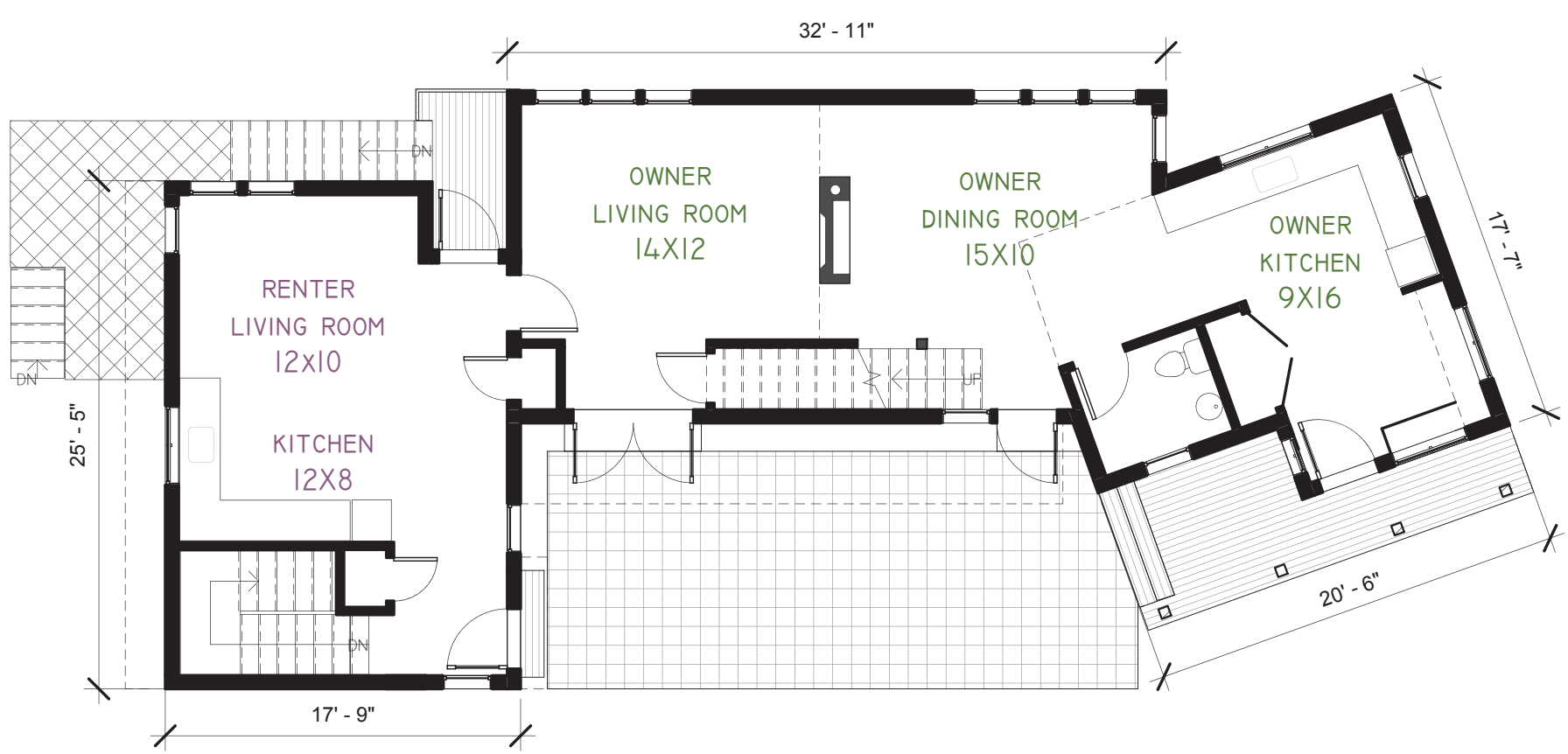
LEVEL 1 - OWNER & RENTER 1/8" SCALE
